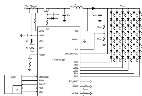
Simplified Schematic
