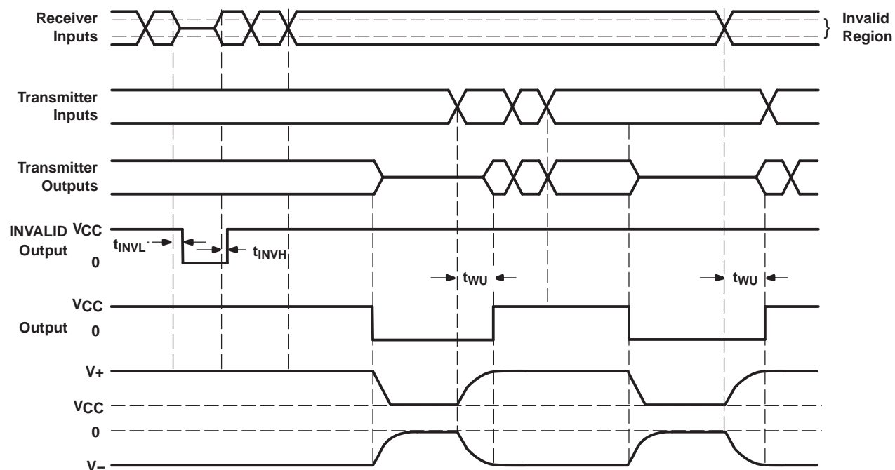
VOLTAGE WAVEFORMS
