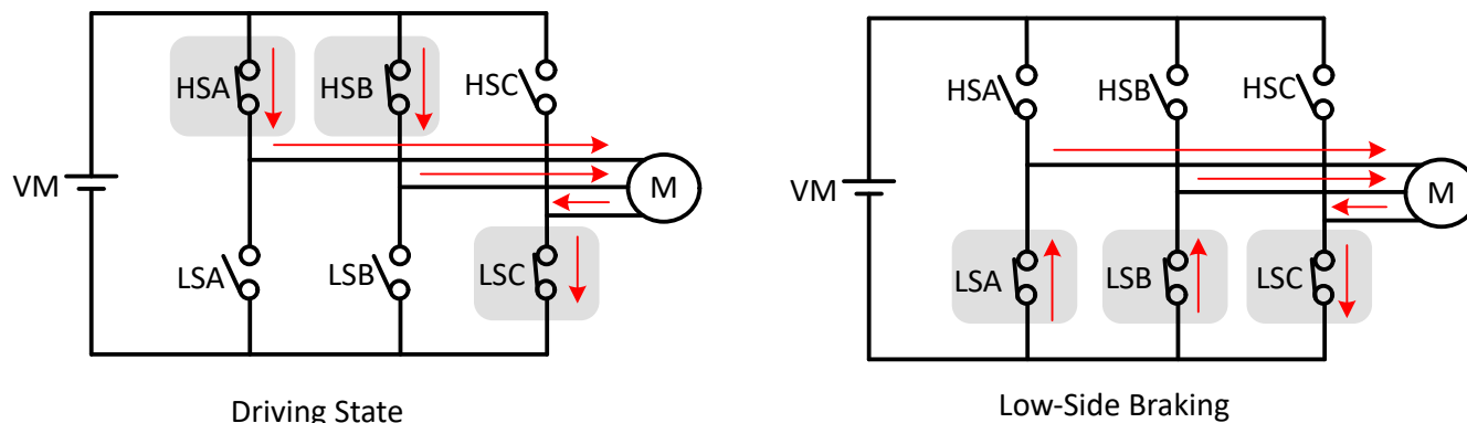
Figure 7-56. Low-Side Braking
