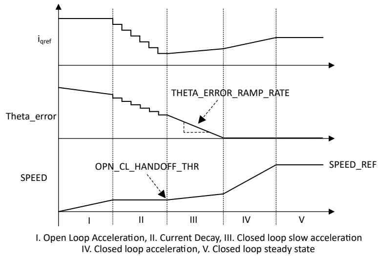
Figure 7-36. Control Sequence in Open to Closed Loop Transition
