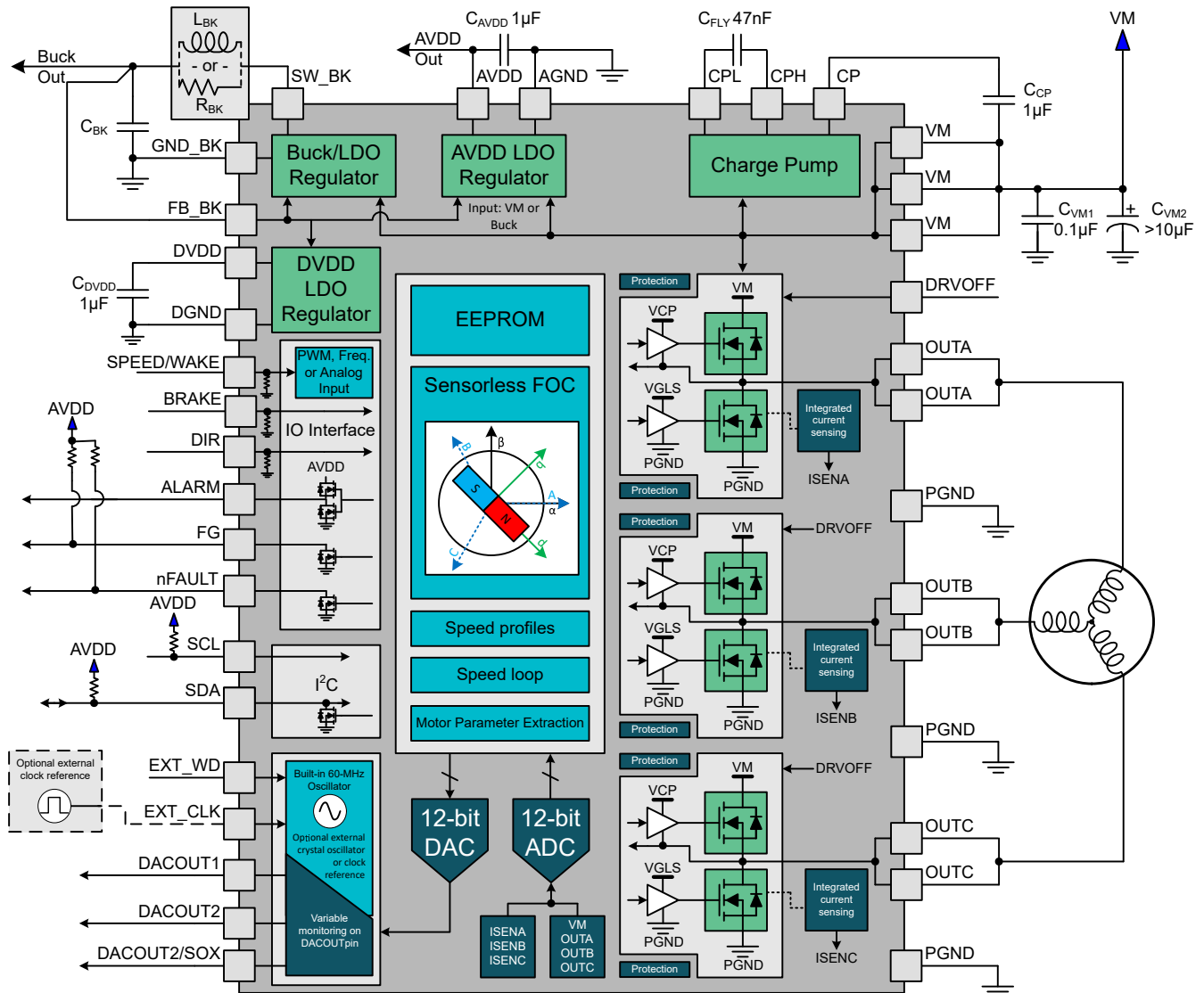
Figure 7-1. MCF8316D Functional Block Diagram
