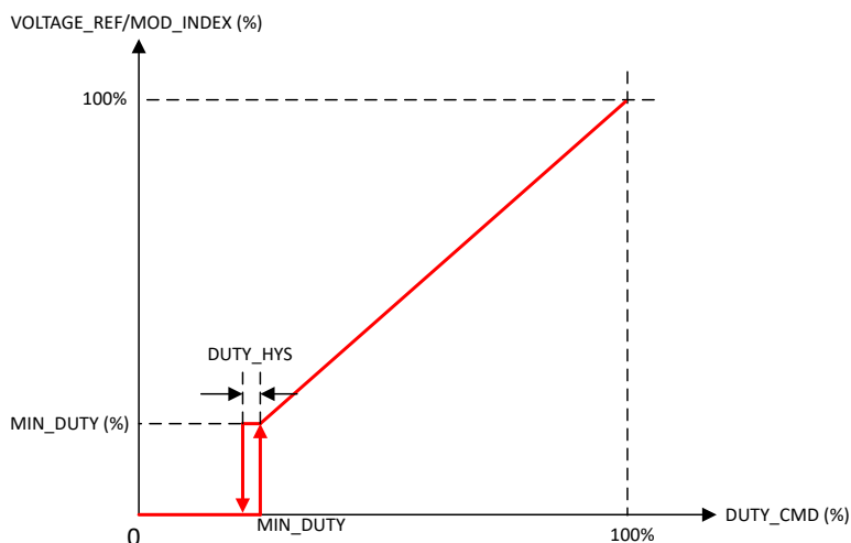
Figure 7-25. Voltage Reference Transfer Function
