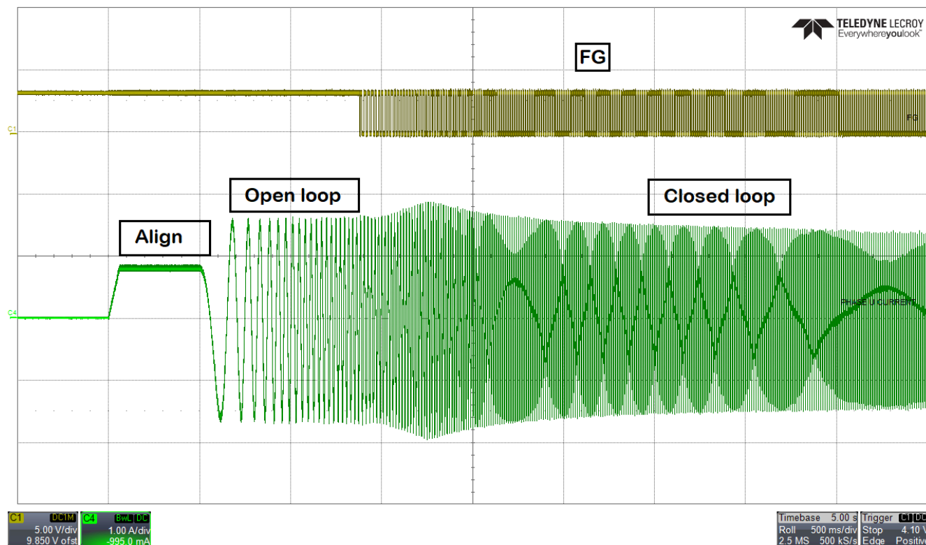
Figure 10-2. Motor Startup - FG and Phase current
