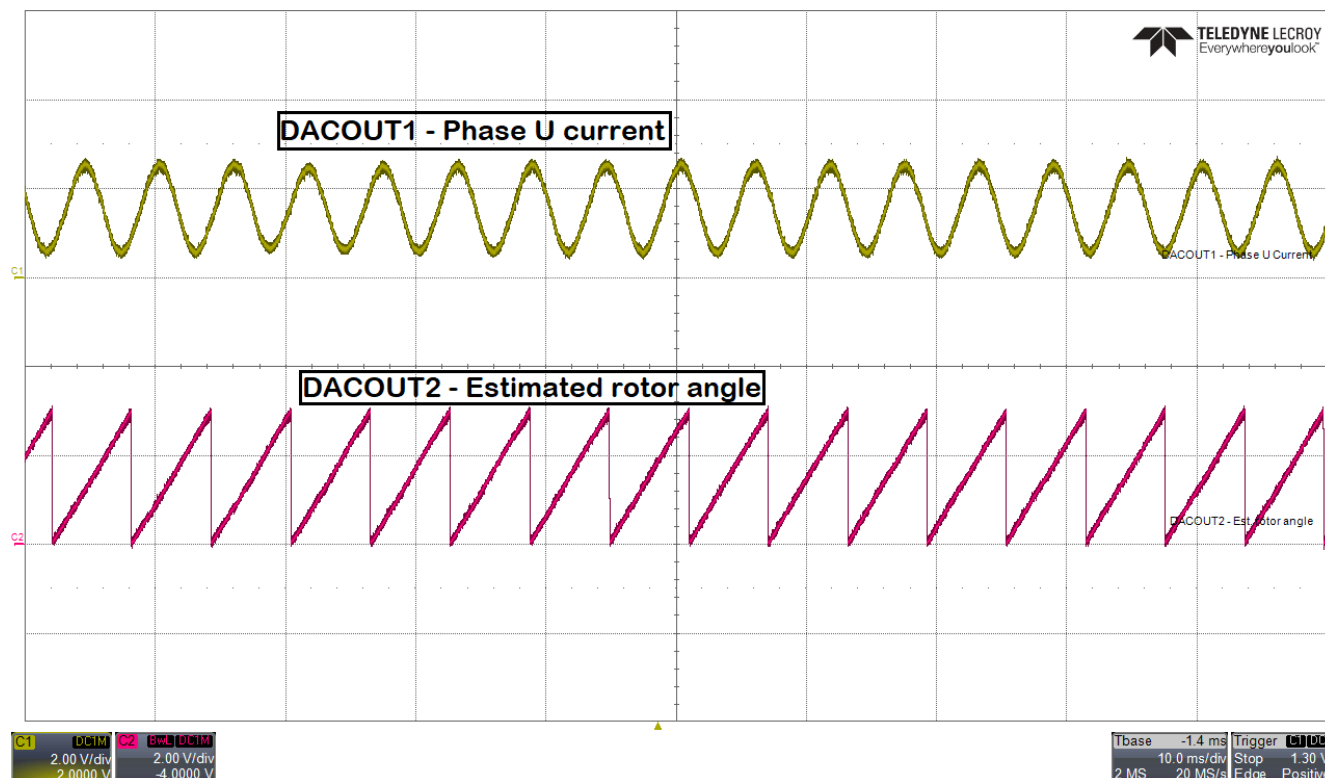
Figure 10-10. DACOUT1 and DACOUT2
