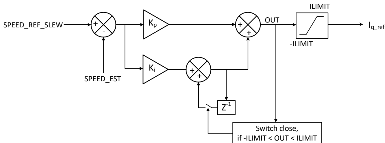
Figure 7-40. Speed PI Control
