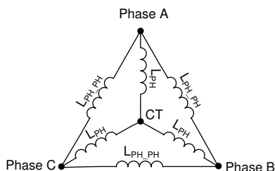
Figure 7-47. Motor Inductance
