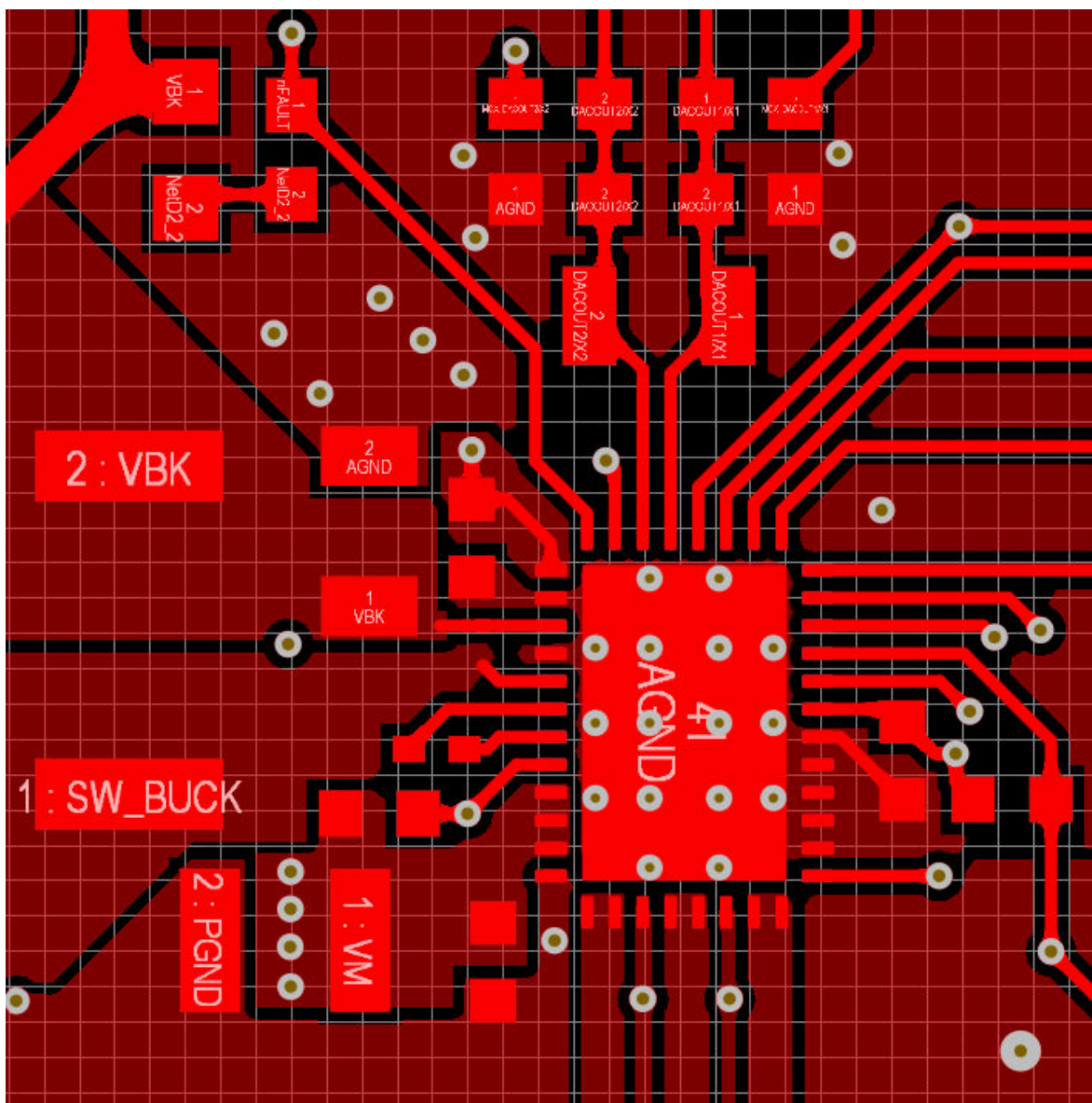
Figure 10-13. Recommended Layout Example
