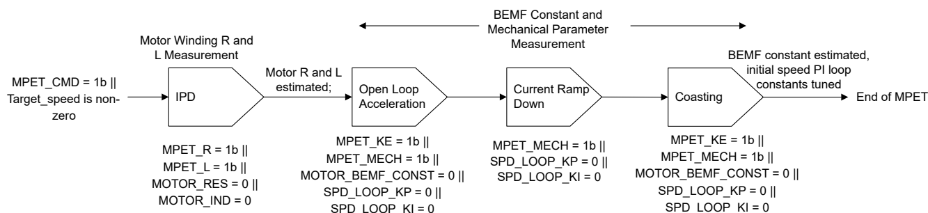
Figure 7-49. MPET Sequence
