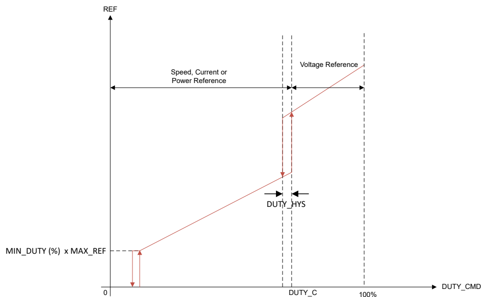
Figure 7-21. Multi-Reference Mode Operation (when VOLTAGE_MODE_CONFIG = 01b)
