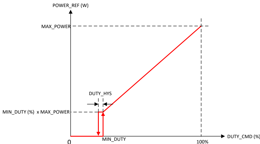
Figure 7-24. Power Reference Transfer Function
