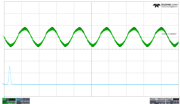
Figure 10-6. Phase current and FFT - Dead time compensation enabled
