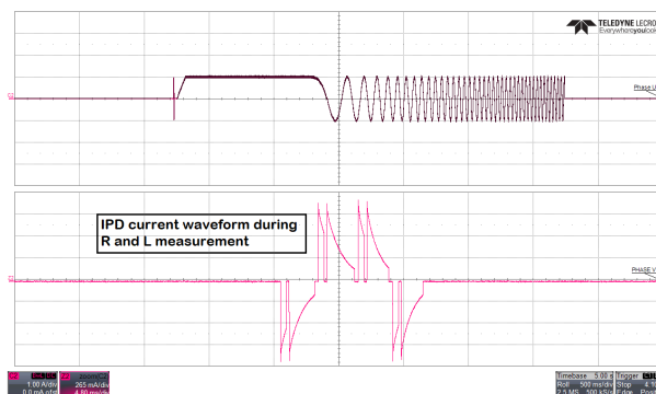
Figure 10-4. IPD current waveform during R and L measurement
