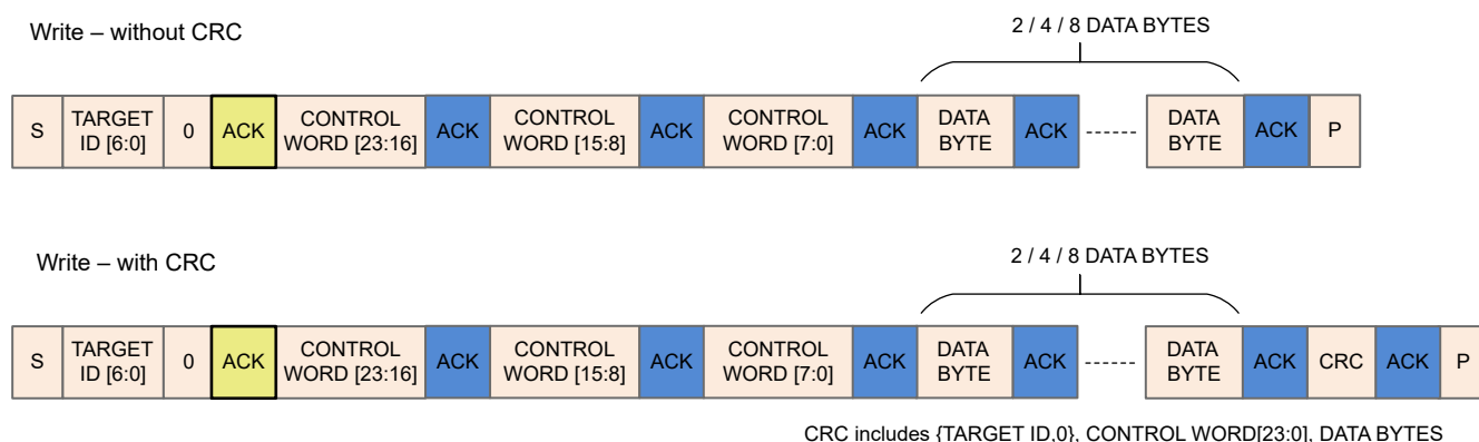
Figure 7-65. I 2 C Write Transaction Sequence
