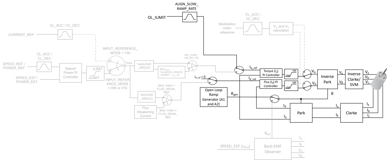
Figure 7-35. Open Loop
