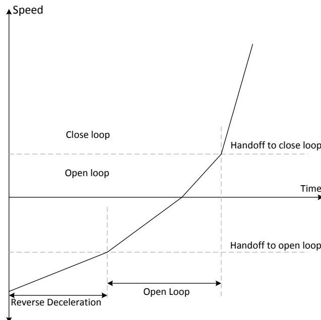
Figure 7-30. Reverse Drive Function
