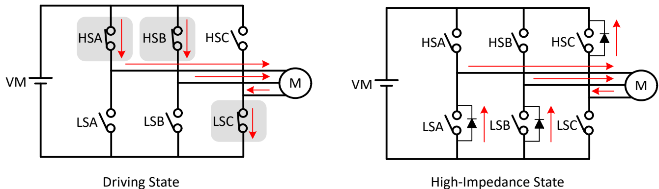
Figure 7-53. Coast (Hi-Z) Mode
