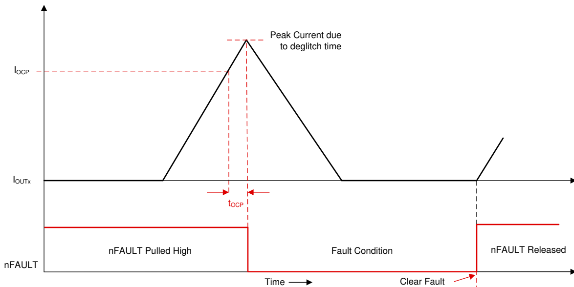
Figure 7-62. Overcurrent Protection - Latched Shutdown Mode
