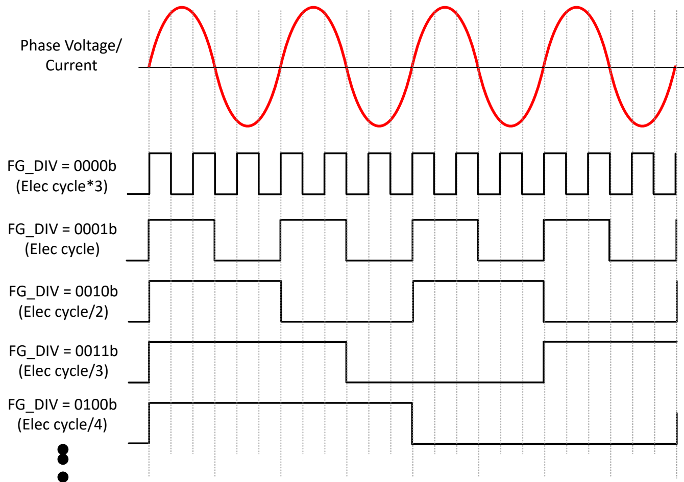
Figure 7-58. FG Frequency Divider
