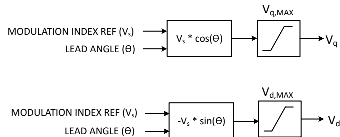
Figure 7-44. Open Loop Voltage Control
