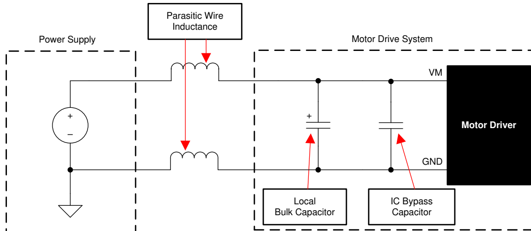
Figure 10-12. Example Setup of Motor Drive System With External Power Supply
