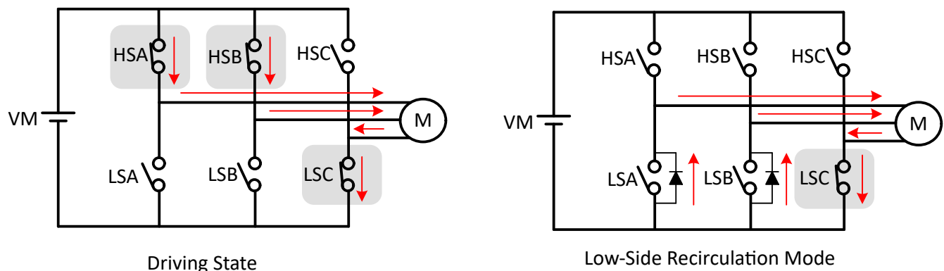
Figure 7-54. Low-Side Recirculation
