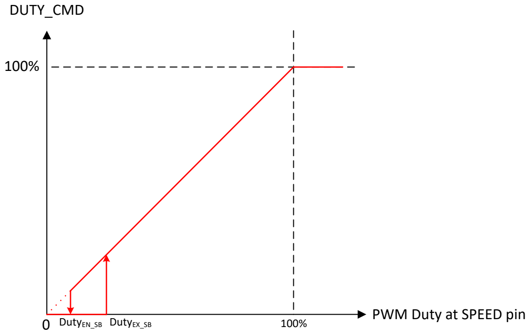
Figure 7-15. PWM-Mode Motor Control
