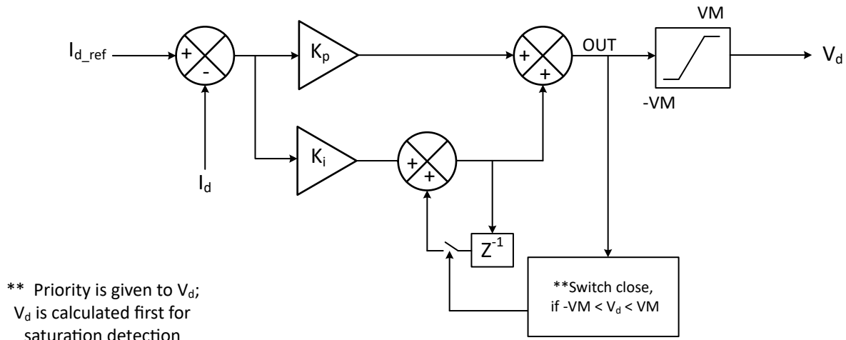
Figure 7-41. I_d Current PI Control
