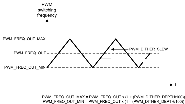
Figure 7-51. Triangular PWM Dithering
