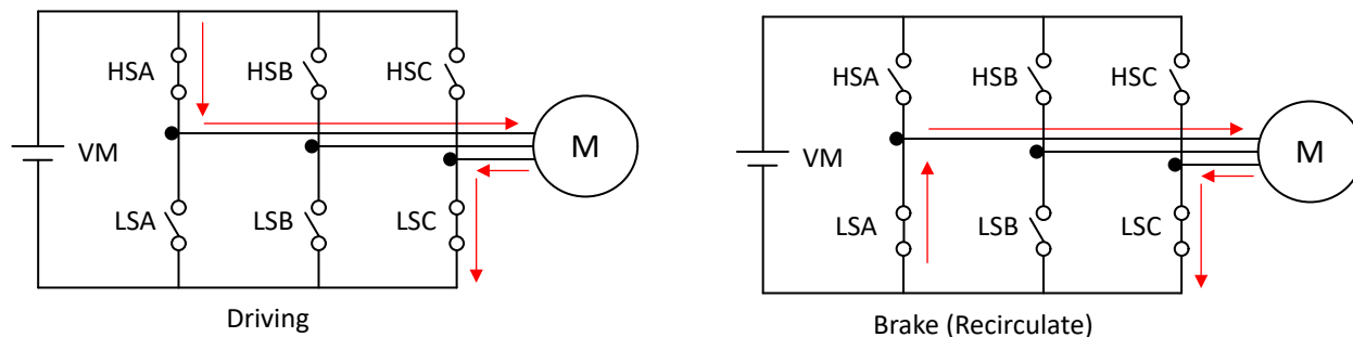
Figure 7-32. IPD Release Mode - Brake (0b)
