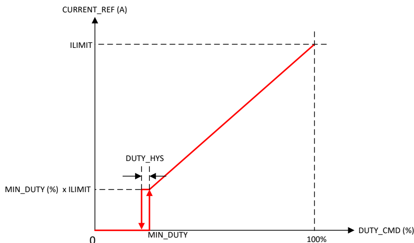
Figure 7-26. Current Reference Transfer Function
