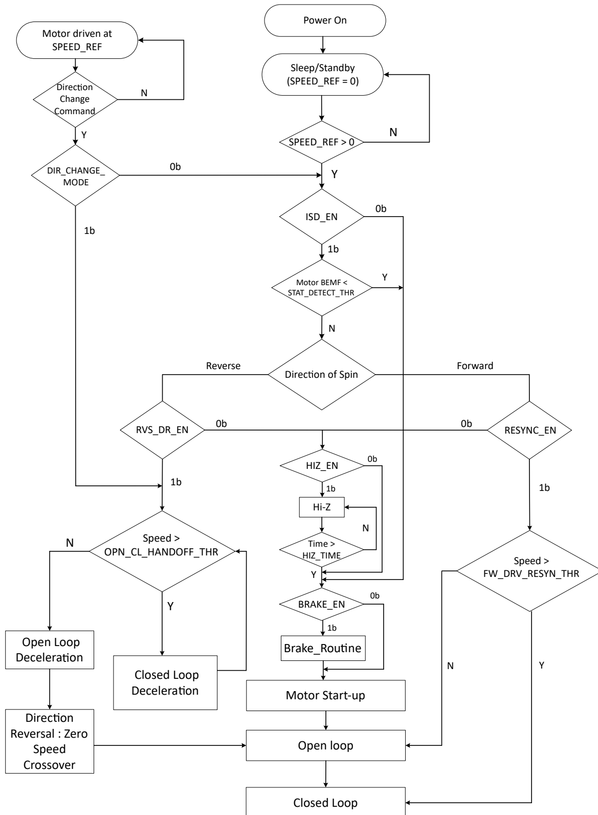
Figure 7-28. Motor Start Sequence
