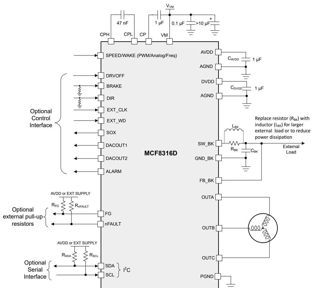
Figure 10-1. Example Application Schematic
