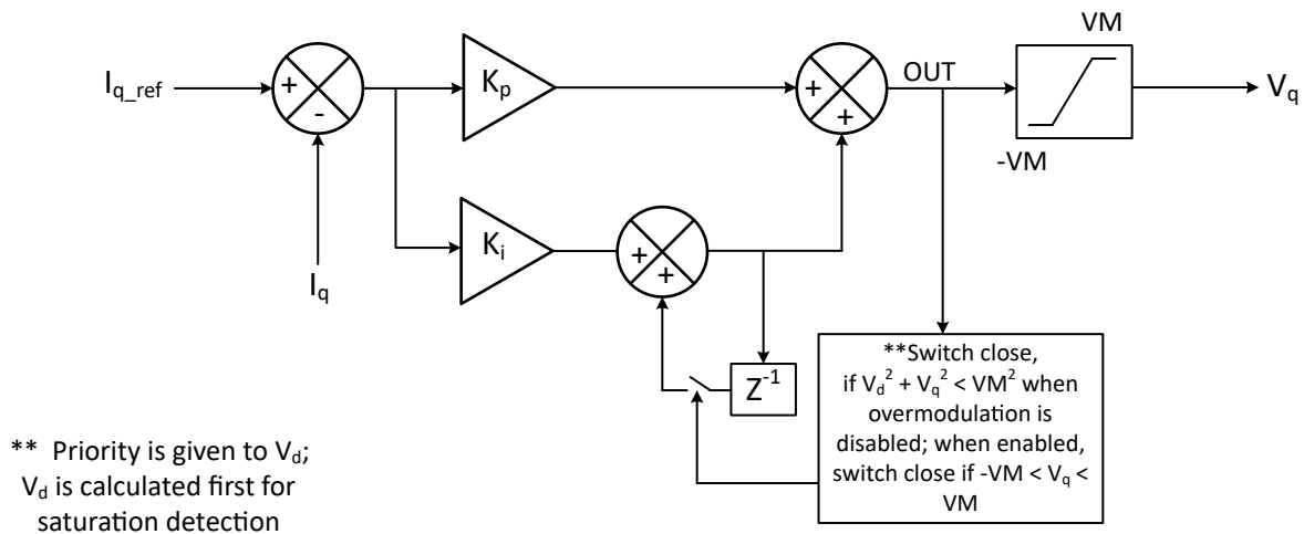
Figure 7-42. I_q Current PI Control
