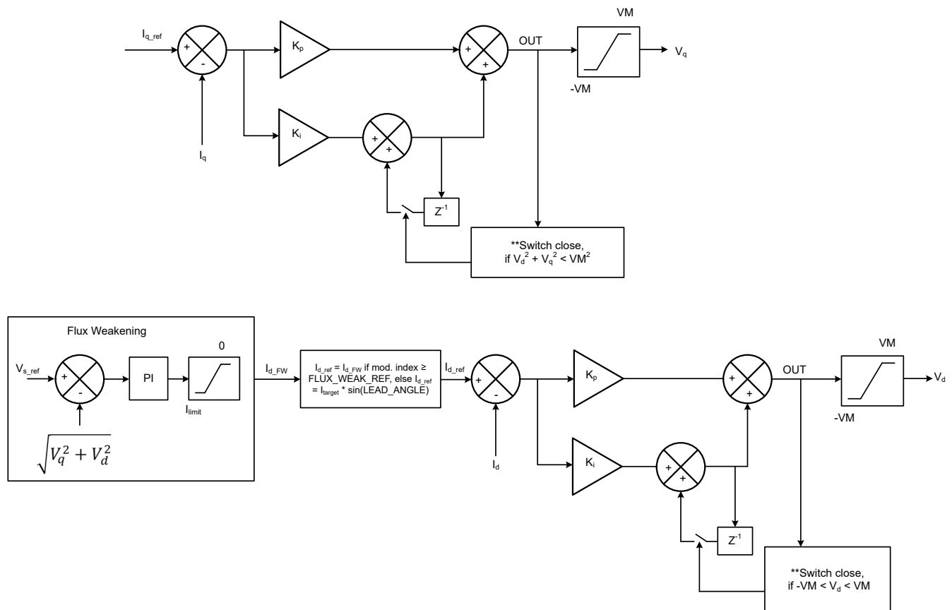
Figure 7-45. Flux Weakening Control
