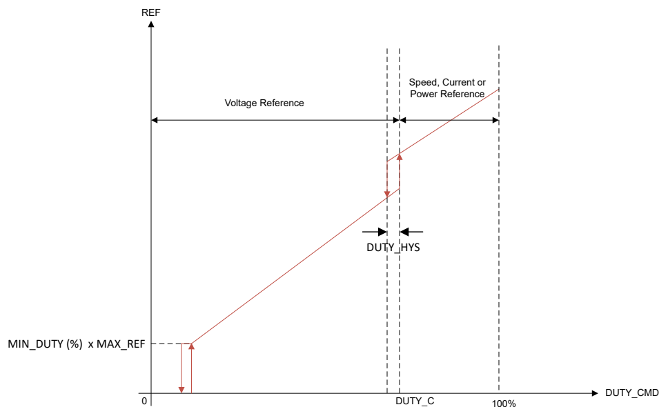
Figure 7-22. Multi-Reference Mode Operation (when VOLTAGE_MODE_CONFIG = 10b)
