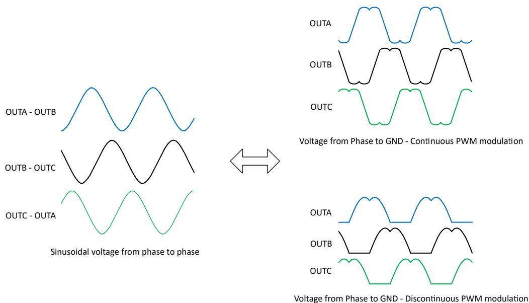
Figure 7-52. Continuous and Discontinuous PWM Modulation Phase Voltages
