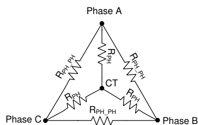
Figure 7-46. Motor Resistance
