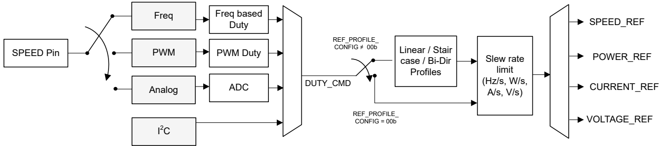
Figure 7-13. Multiplexing the Reference Input Command
