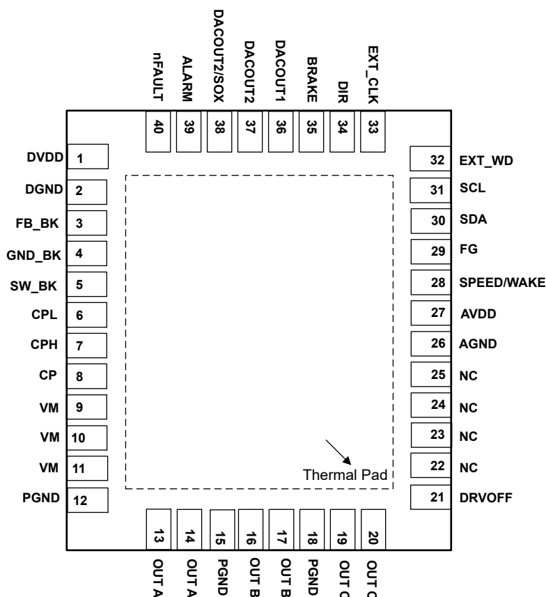
Figure 5-1. MCF8316D, 40-Pin VQFN With Exposed Thermal Pad, Top View
