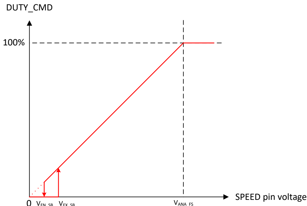
Figure 7-14. Analog-Mode Motor Control
