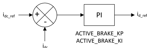
Figure 7-50. Active Braking Current Control Loop for i_{d\_ref}
