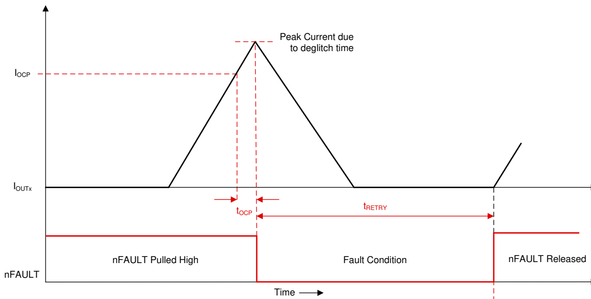
Figure 7-63. Overcurrent Protection - Automatic Retry Mode
