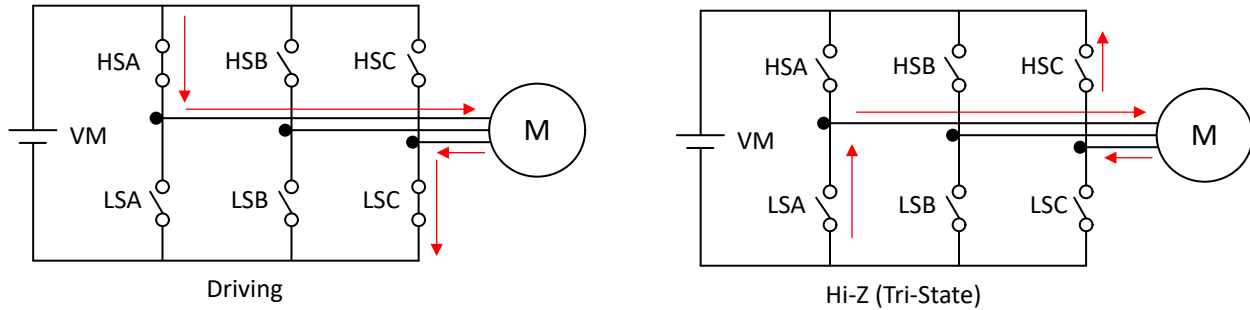
Figure 7-33. IPD Release Mode - Tristate (1b)
