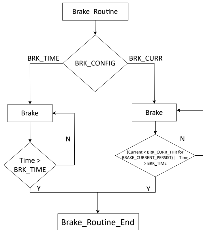
Figure 7-29. Brake Routine
