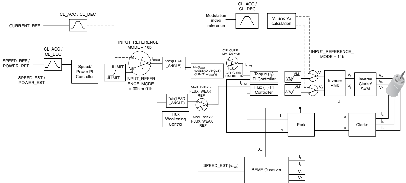
Figure 7-38. Closed Loop FOC Control
