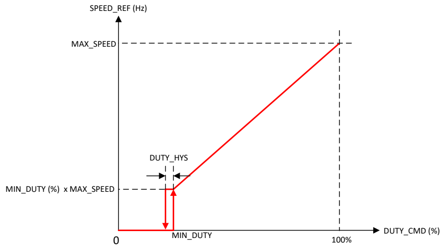
Figure 7-23. Speed Reference Transfer Function
