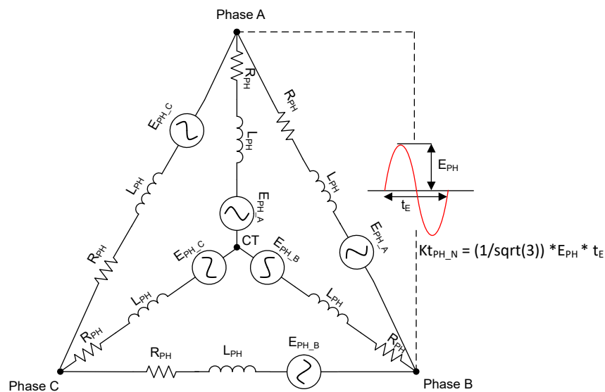
Figure 7-48. Motor back-EMF constant
