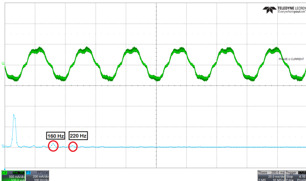
Figure 10-5. Phase current and FFT - Dead time compensation disabled
