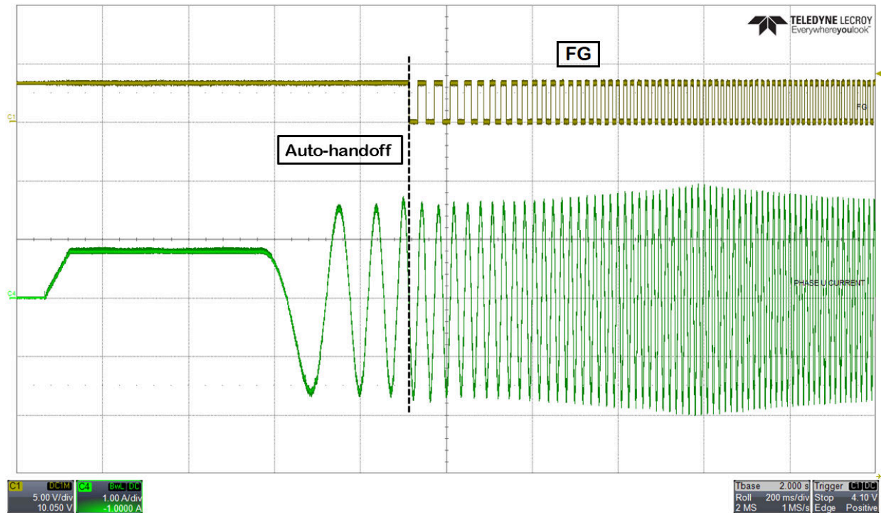
Figure 10-7. Auto-handoff
