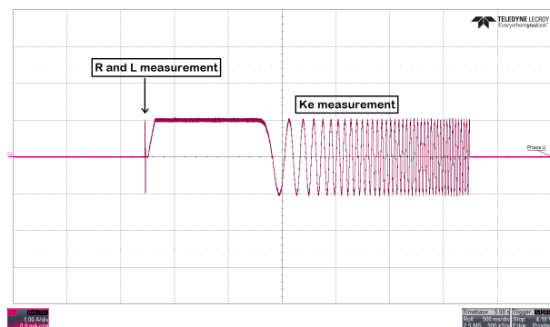
Figure 10-3. MPET - Phase current
