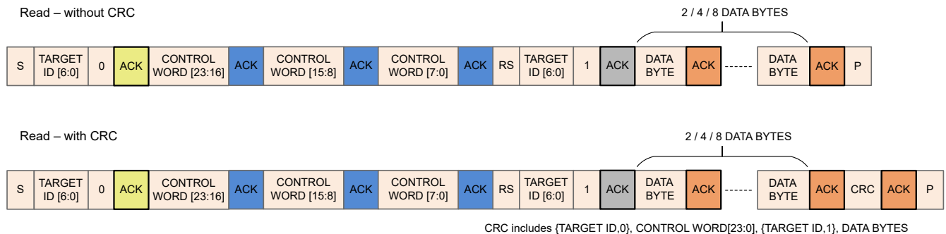
Figure 7-66. I 2 C Read Transaction Sequence
