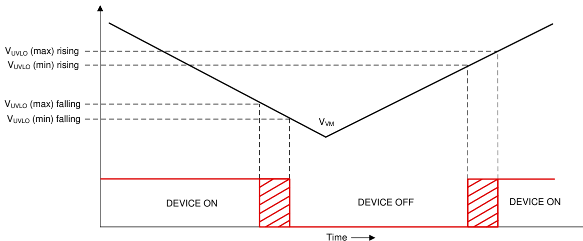
Figure 7-60. VM Supply Undervoltage Lockout
