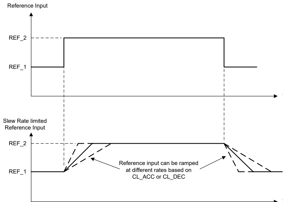
Figure 7-39. Closed Loop Acceleration/Deceleration Slew Rate
