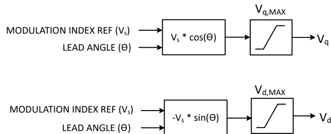
Figure 7-36. Open Loop Voltage Control
