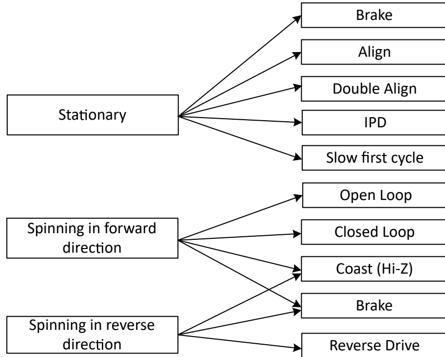
Figure 7-21. Starting the motor under different initial conditions
