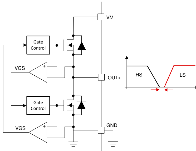
Figure 8-18. Cross Conduction Protection
