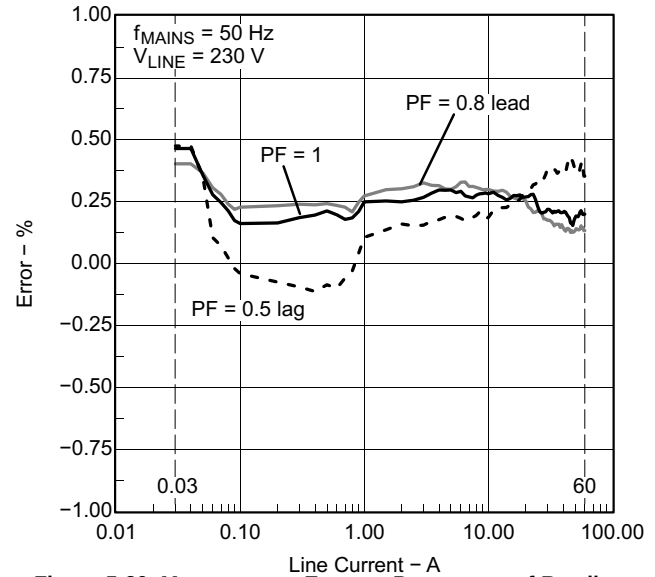
Figure 5-20. Measurement Error as Percentage of Reading ( T_A = -40^{\circ}\text{C} )
