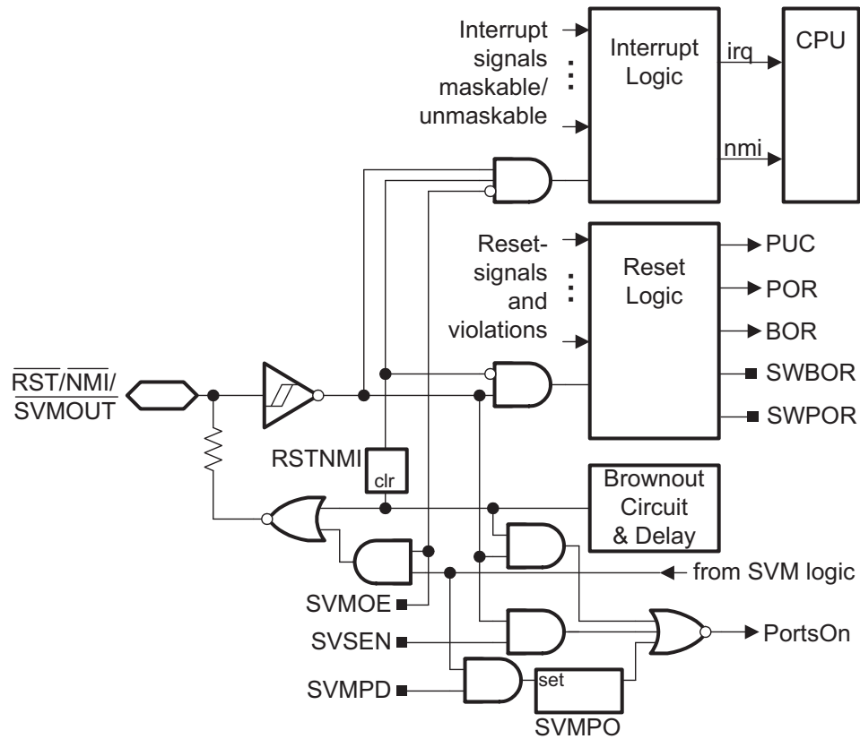
Figure 2. \overline{\text{RST}}/\overline{\text{NMI}}/\overline{\text{SVMOUT}} and PortsOn Logic Block Diagram
