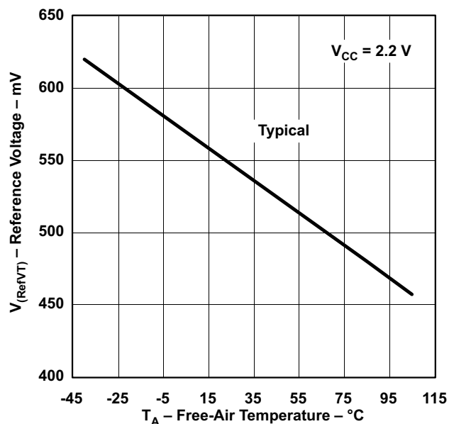
Figure 25. V (RefVT) vs Temperature, V CC = 2.2 V
