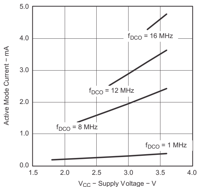
Figure 5. Active Mode Current vs V_{CC} , T_A = 25^\circ C
