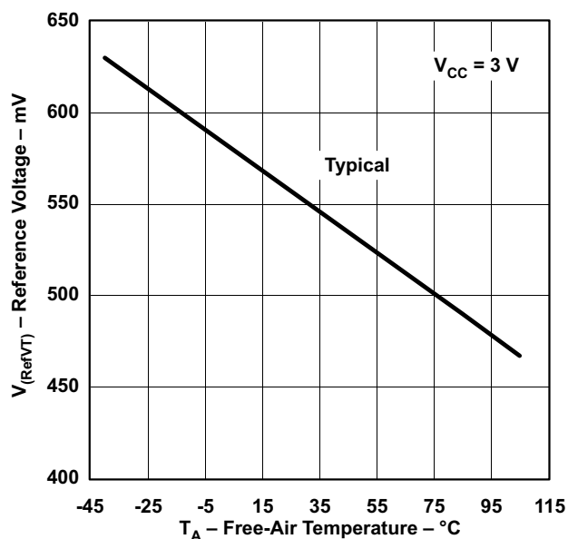
Figure 24. V (RefVT) vs Temperature, V CC = 3 V
