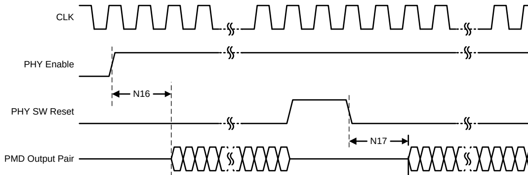
Figure 5-35. Reset Timing
