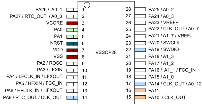
Figure 6-3. 28-Pin DGS28 (VSSOP) (Top View)
