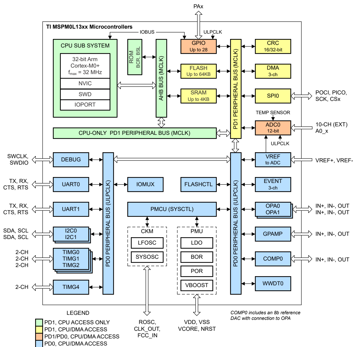
Figure 4-1. MSPM0L134x, MSPM0L130x Functional Block Diagram
