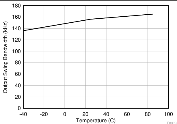
Figure 5-3. Output Swing Bandwidth vs Temperature at V_{CC} = \pm 10 V
