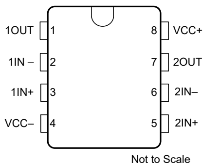
Figure 4-1. NE5532x, D Package, 8-Pin SOIC, P Package, 8-Pin PDIP, PS Package, 8-Pin SO SA5532x, D Package, 8-Pin SOIC, P Package, 8-Pin PDIP (Top View)
