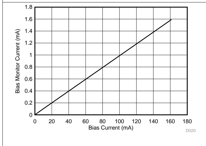
Figure 12. Bias-Monitor Current I_{(MONB)} vs Bias Current
