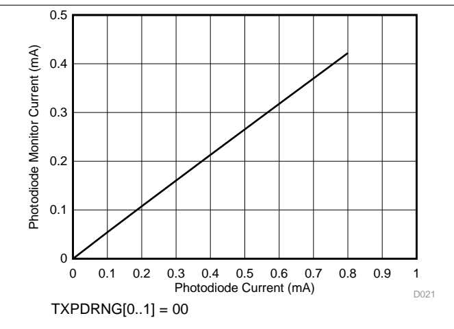
Figure 13. Photodiode-Monitor Current I_{(MONP)} vs PD Current
