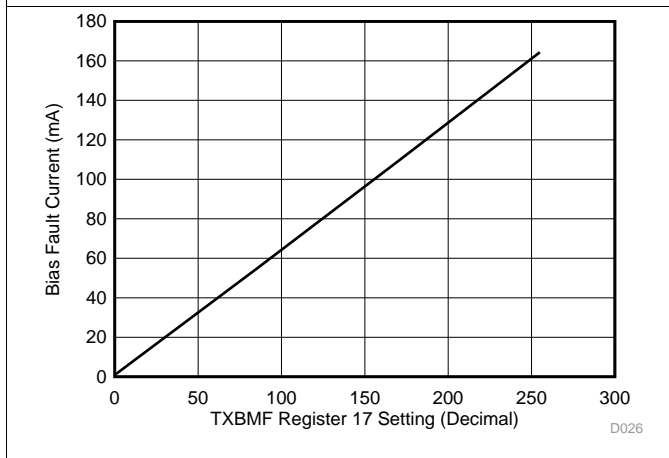
Figure 18. Bias Current Monitor Fault vs TXBMF Register Setting
