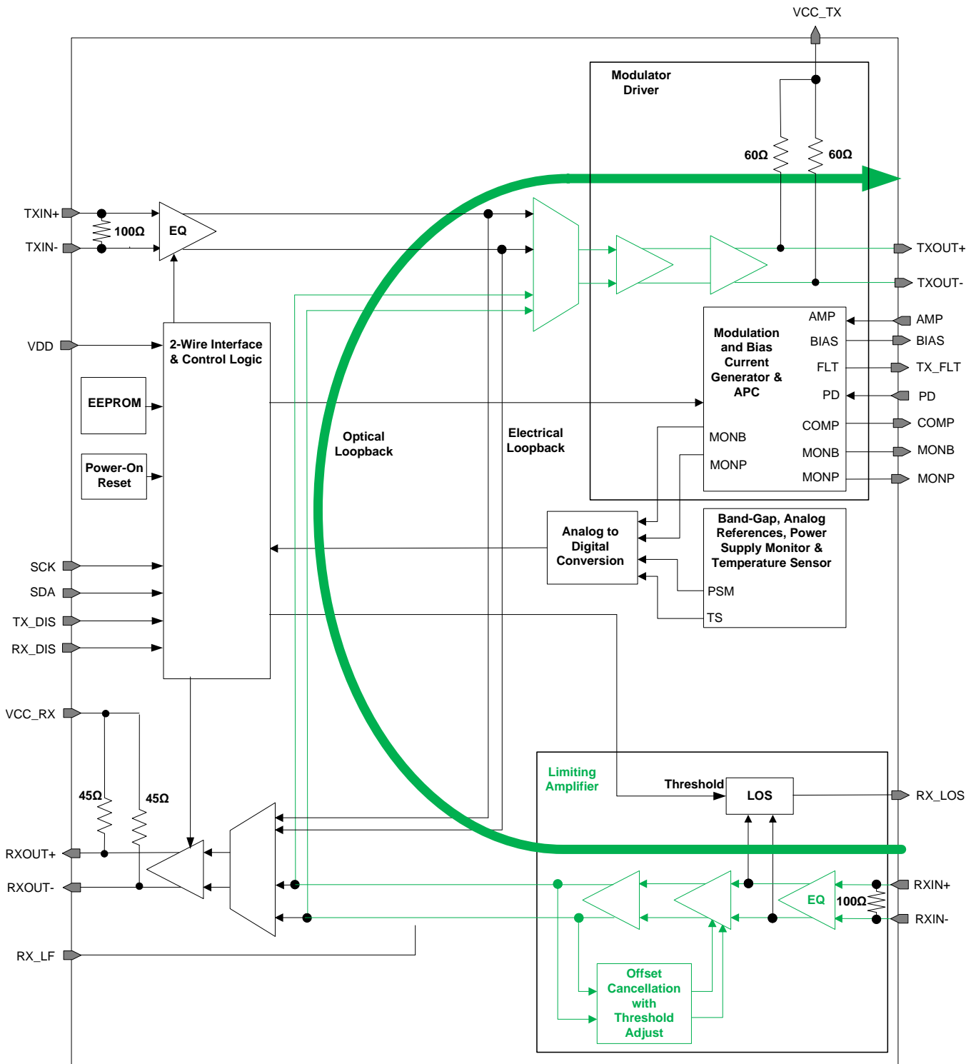
Figure 36. Optical Loopback
