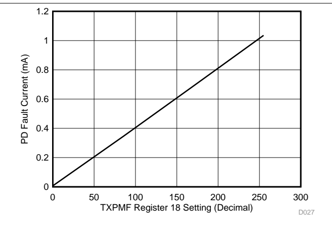
Figure 19. Photodiode Current Monitor Fault vs TXPMF Register Setting
