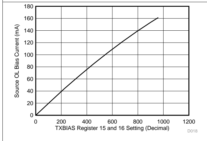
Figure 10. Source Bias Current in Open Loop Mode vs Bias Register Setting
