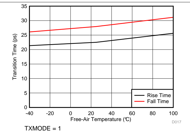
Figure 9. TX Rise-Time and Fall-Time vs Temperature
