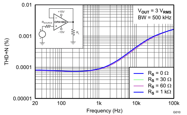
Figure 5-10. THD+N Ratio vs Frequency
