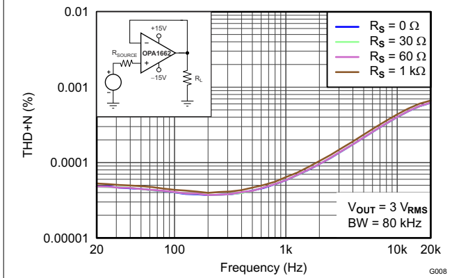
Figure 5-9. THD+N Ratio vs Frequency
