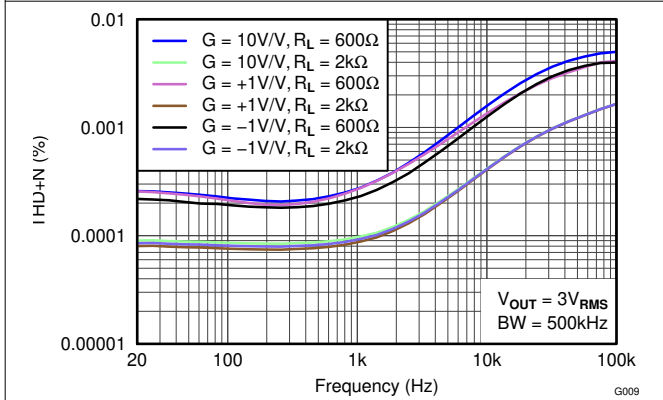
Figure 5-7. THD+N Ratio vs Frequency
