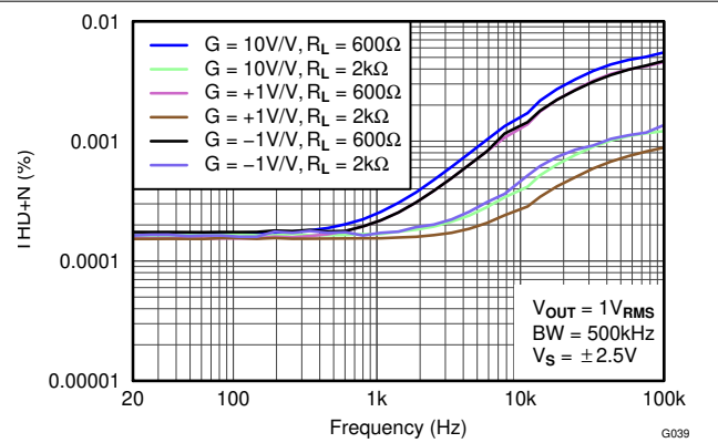
Figure 5-8. THD+N Ratio vs Frequency
