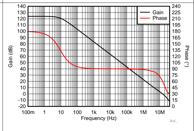
Figure 6. Open-Loop Gain and Phase vs Frequency
