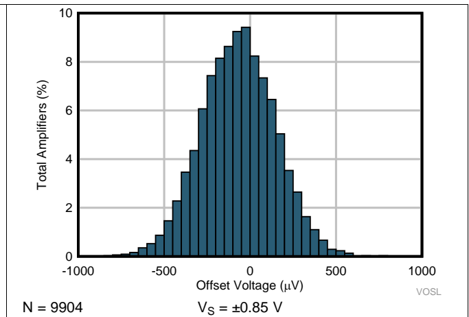
Figure 2. Offset Voltage Production Distribution
