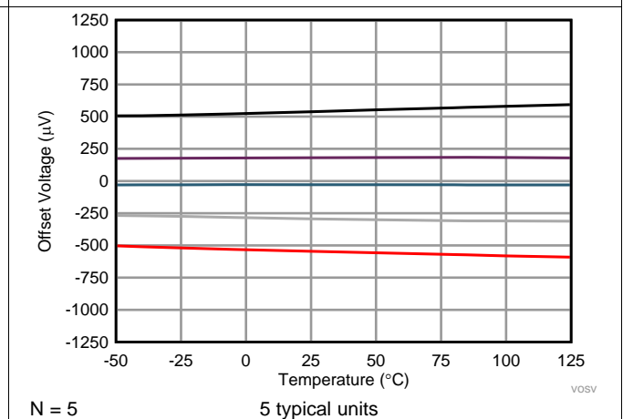
Figure 4. Offset Voltage vs Temperature
