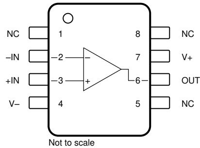
Figure 4-1. OPA206: D Package, 8-Pin SOIC (Top View)
