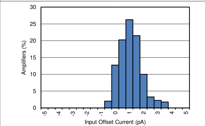
Figure 6-4. Input Offset Current Production Distribution
