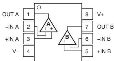
Pin Functions
