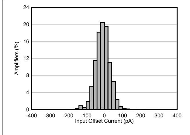
Figure 6-21. Input Offset Current Production Distribution
