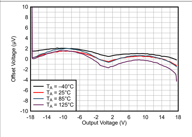
Figure 6-6. Offset Voltage vs Output Voltage
