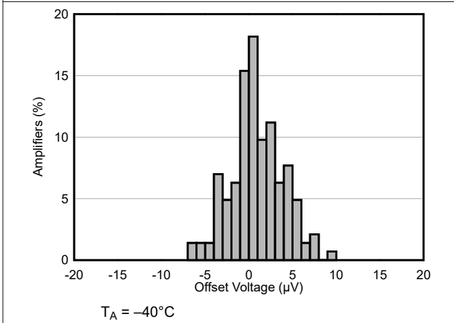
Figure 6-3. Offset Voltage Distribution at -40°C
