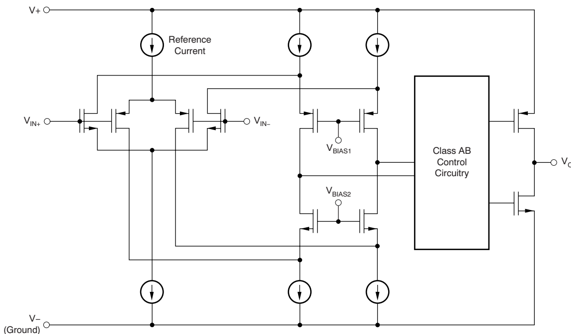
Figure 34. Simplified Schematic
