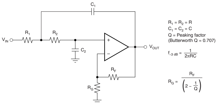
Figure 38. Two-Pole Low-Pass Sallen-Key Filter
