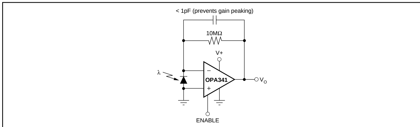
FIGURE 7. Transimpedance Amplifier.
