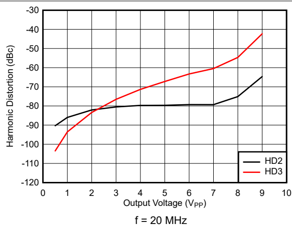
Figure 7-10. Harmonic Distortion vs Output Voltage
