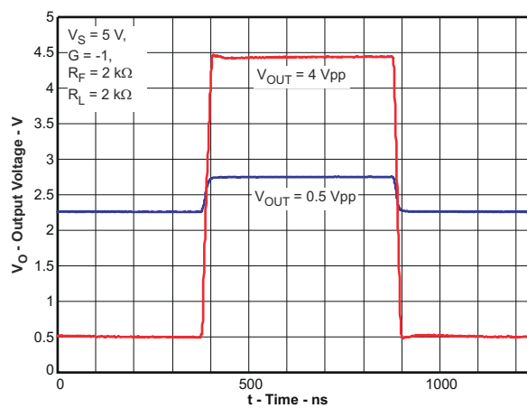
Figure 7-30. Inverting Pulse Response
