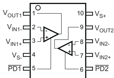
Figure 6-3. OPA2835: DGS Package 10-Pin VSSOP Top View
