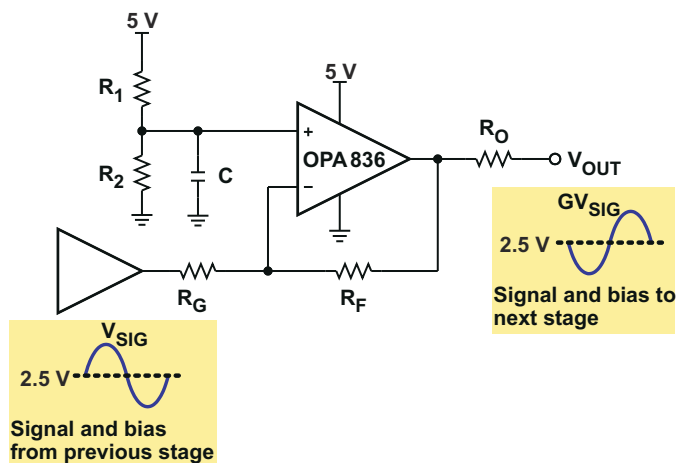
Figure 8-11. Inverting Single Supply With Resistors
