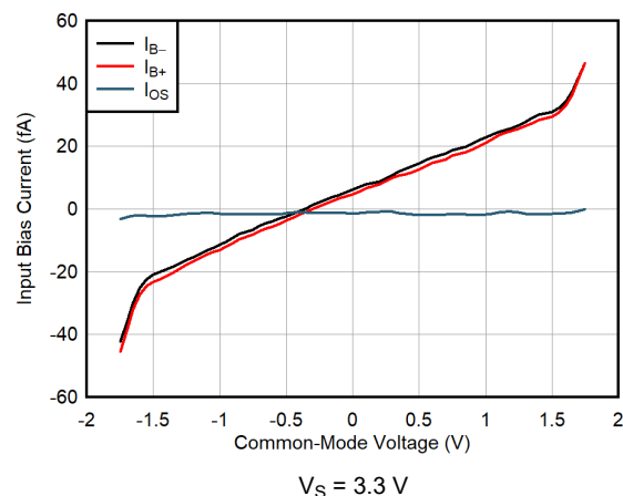
Figure 6-12. Input Bias Current vs Common-Mode Voltage
