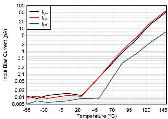
Figure 6-14. Input Bias Current vs Temperature
