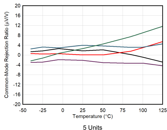
Figure 6-20. CMRR vs Temperature
