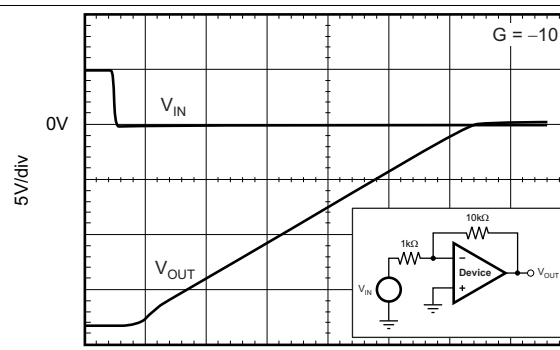
Figure 28. Negative Overload Recovery
