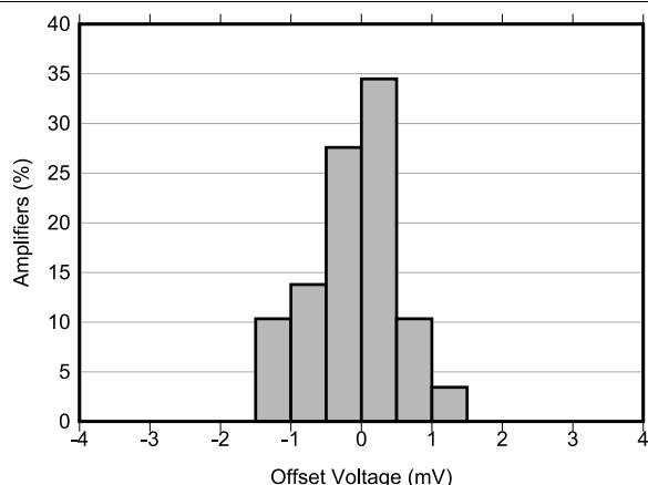
Figure 6-1. Offset Voltage Distribution at 25^\circ\text{C}
