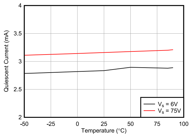
Figure 6-55. Quiescent Current vs Temperature
