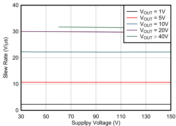
Figure 6-44. Slew Rate vs Supply Voltage (Inverting)
