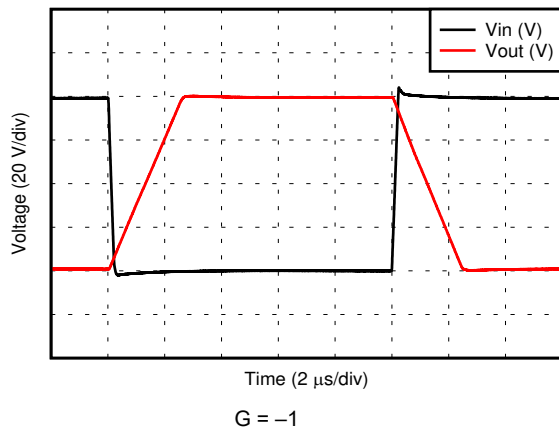
Figure 6-41. Large-Signal Step Response
