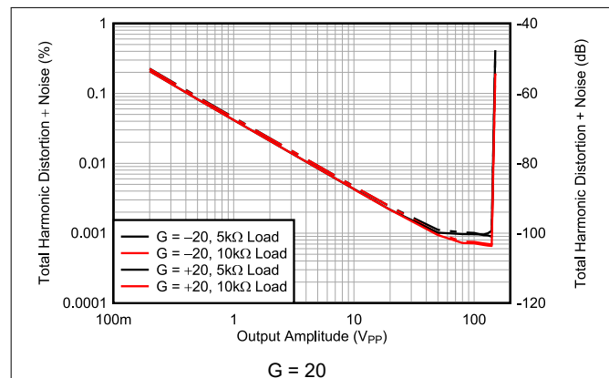
Figure 6-49. THD+N Ratio vs Output Amplitude
