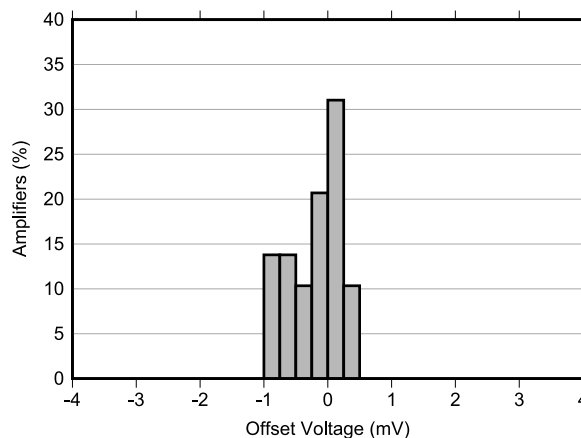
Figure 6-2. Offset Voltage Distribution at 85^\circ\text{C}
