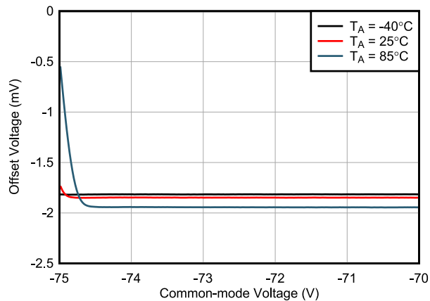
Figure 6-7. Offset Voltage vs Common-Mode Voltage (Low V_{CM} )
