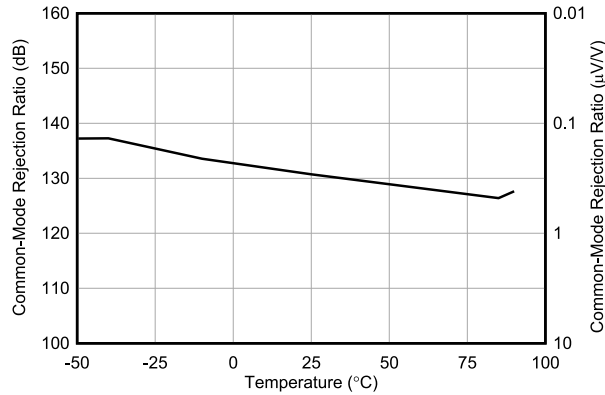
Figure 6-13. CMRR vs Temperature
