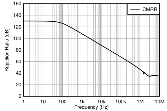
Figure 6-14. CMRR vs Frequency
