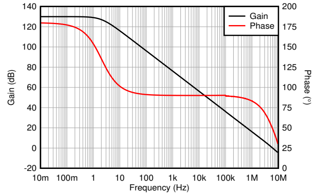
Figure 6-26. Open-Loop Gain and Phase vs Frequency
