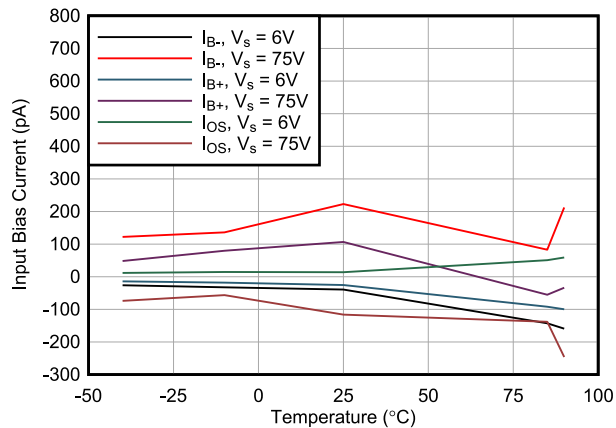
Figure 6-20. IB vs Temperature
