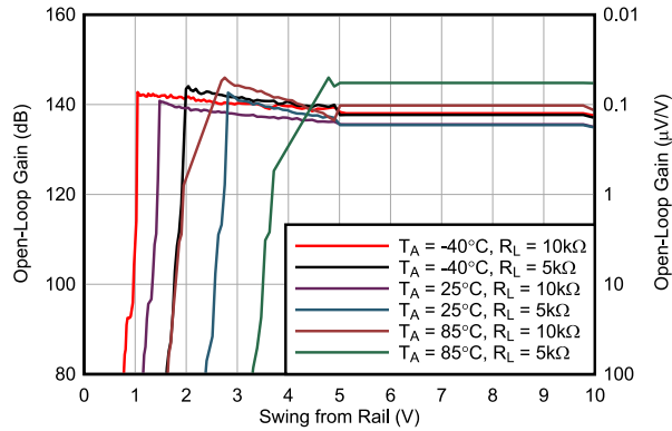
Figure 6-25. Open-Loop Gain vs Output Voltage
