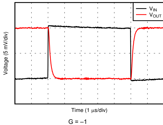
Figure 6-39. Small-Signal Step Response
