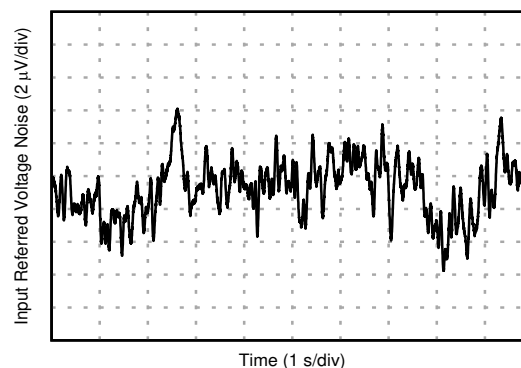
Figure 6-50. 0.1-Hz to 10-Hz Noise
