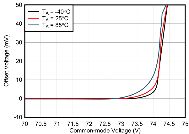
Figure 6-8. Offset Voltage vs Common-Mode Voltage (High V_{CM} )
