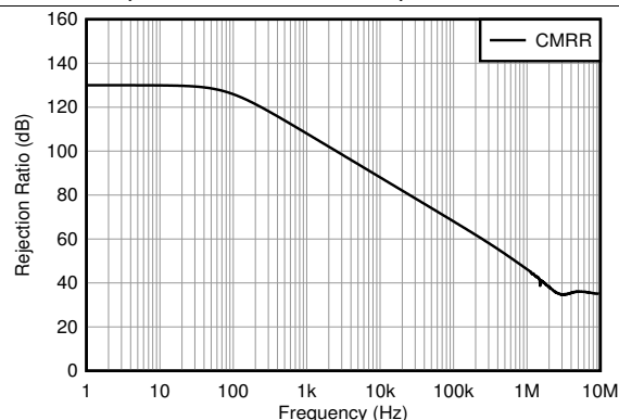
Figure 14. CMRR vs Frequency
