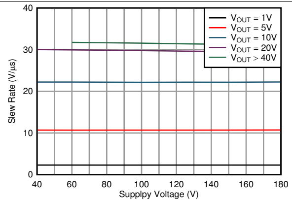
Figure 44. Slew Rate vs Supply Voltage (Inverting)
