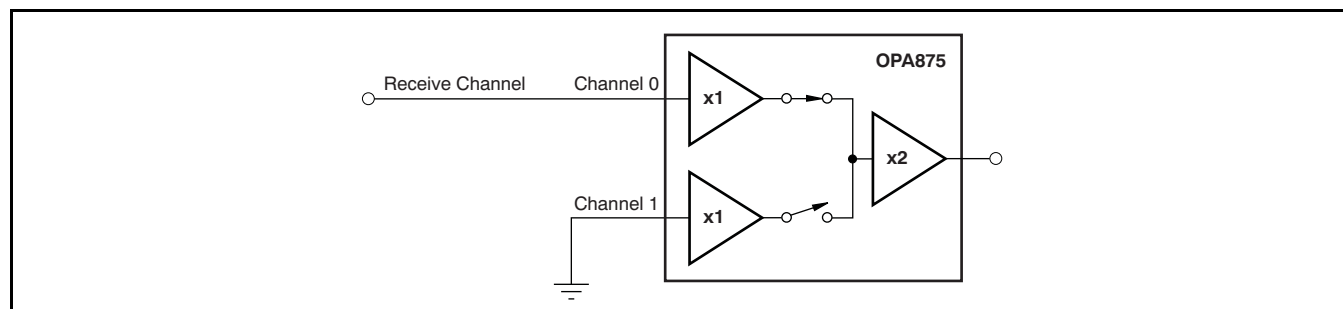
Figure 26. Transmit/Receive Switch
