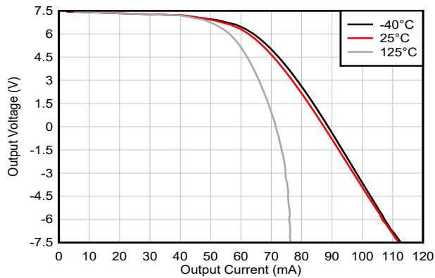
Figure 5-15. Output Voltage Swing vs Output Current (Sourcing) V_S = 15\text{ V}
