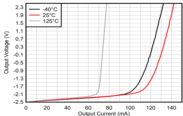
Figure 5-18. Output Voltage Swing vs Output Current (Sinking) V_S = 5\text{ V}
