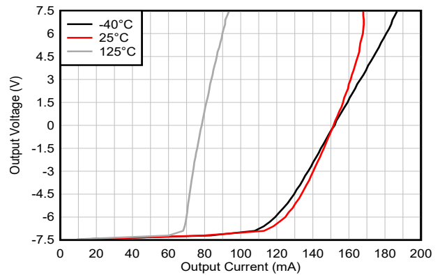
Figure 5-16. Output Voltage Swing vs Output Current (Sinking) V_S = 15\text{ V}
