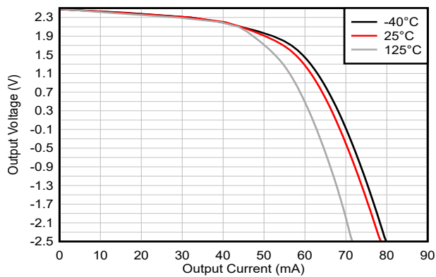
Figure 5-17. Output Voltage Swing vs Output Current (Sourcing) V_S = 5\text{ V}
