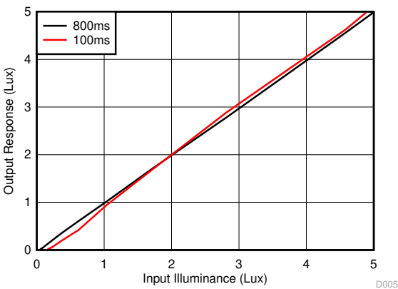
Figure 5-6. Output Response vs Input Illuminance: Low Range = 0lux to 5lux
