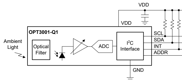
Block Diagram
