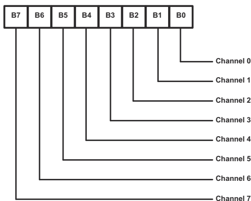
Figure 8-5. Control Register
