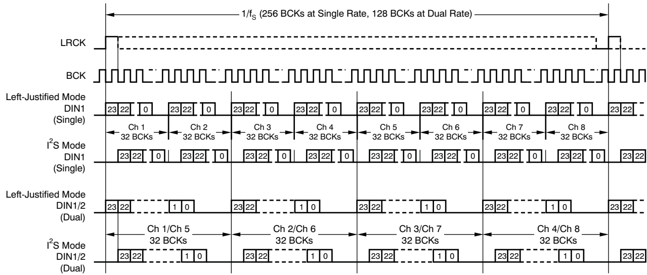
Figure 36. Audio Data Format: 24-Bit TDM Format
