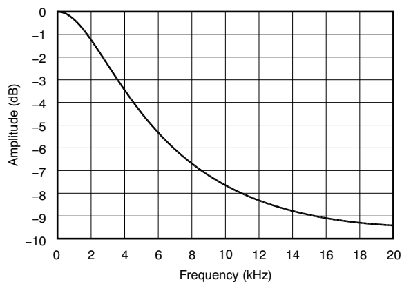
Figure 12. De-emphasis Characteristic
