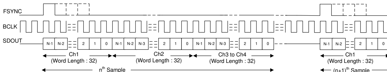
Figure 8-1. TDM Mode Protocol Timing (FMT0 = LOW) In Slave Mode
