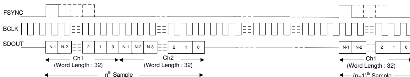
Figure 8-2. TDM Mode Protocol Timing (FMT0 = HIGH) In Slave Mode
