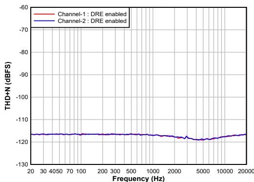
Figure 7-3. Differential Input: DR vs Input Frequency With DRE Enabled
