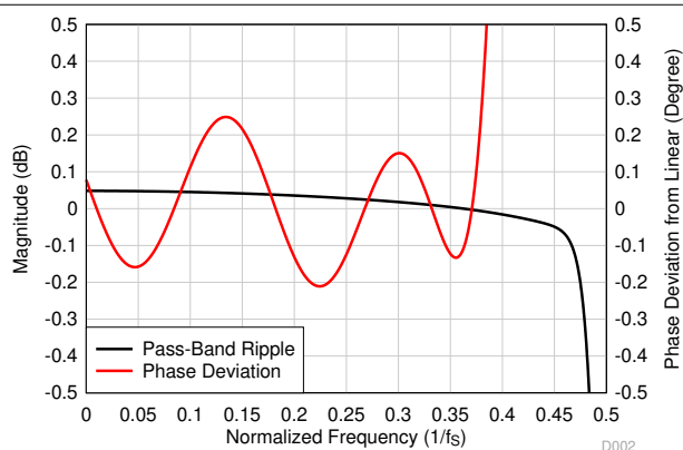
Figure 8-24. Low-Latency Decimation Filter Pass-Band Ripple and Phase Deviation
