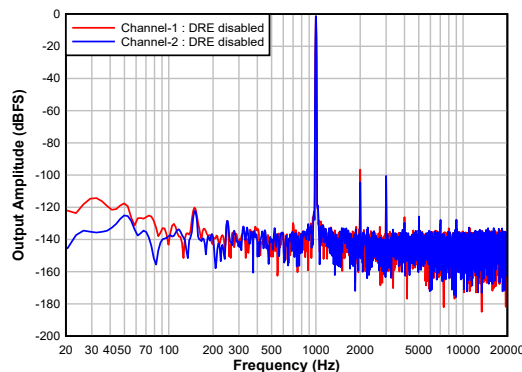
Figure 7-12. Differential Input: FFT With a -1-dBr Input
