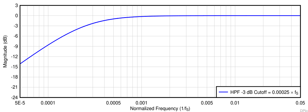
Figure 8-8. HPF Filter Frequency Response Plot
