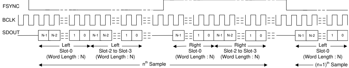
Figure 8-6. I 2 S Mode Standard Protocol Timing (TX_OFFSET = 0)
