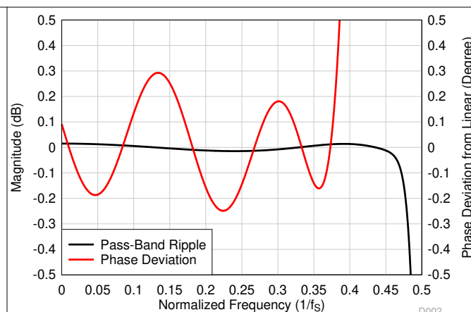
Figure 6-44. Low-Latency Decimation Filter Pass-Band Ripple and Phase Deviation
