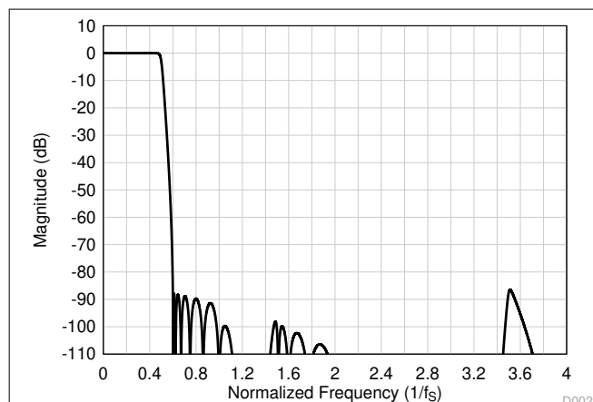
Figure 6-43. Low-Latency Decimation Filter Magnitude Response
