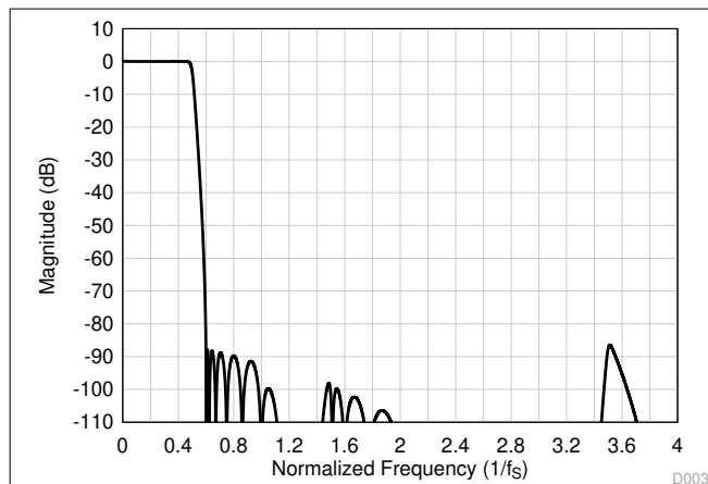
Figure 6-55. Ultra-Low-Latency Decimation Filter Magnitude Response
