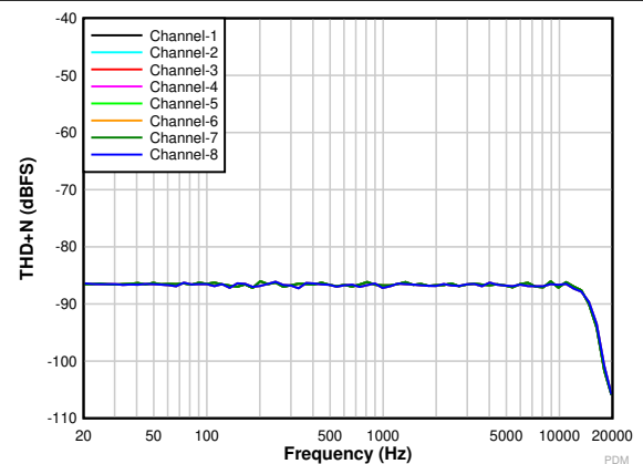
Figure 5-14. THD+N vs Input Frequency With a – 20-dBr Input
