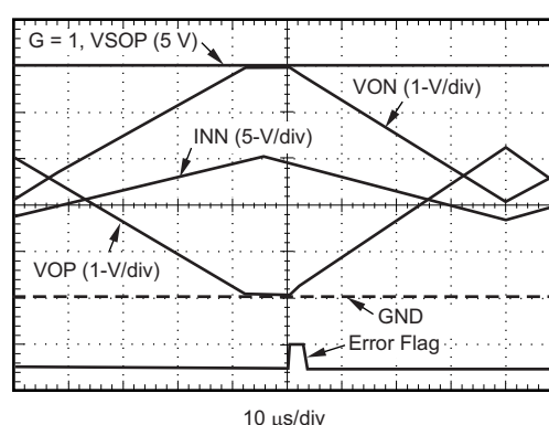
Figure 34. OUTPUT OVERLOAD RECOVERY
