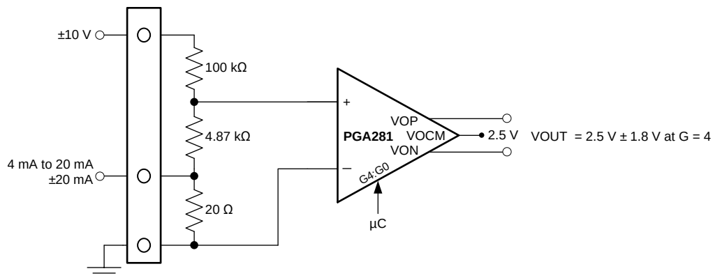
Figure 49. \pm 10\text{-V} , 4-mA to 20-mA PLC Input
