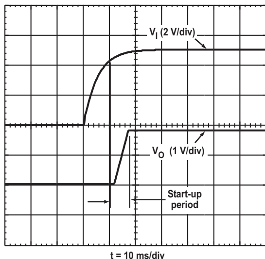
Figure 14. PTV05010W Start-Up
