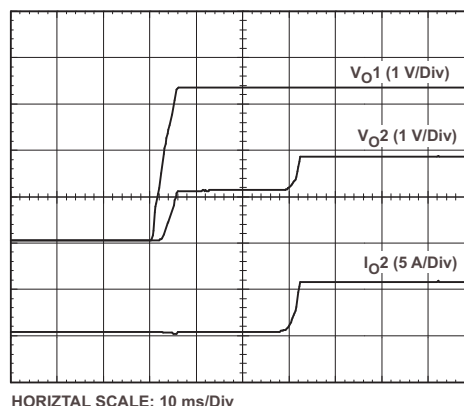
Figure 27. Prebias Startup Waveforms
