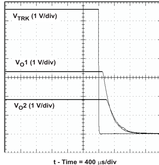
Figure 25. Simultaneous Power Down With Auto-Track Control
