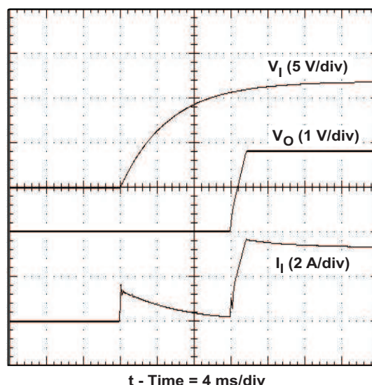
Figure 20. Power-Up Waveform
