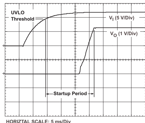
Figure 26. PTH08040W Startup
