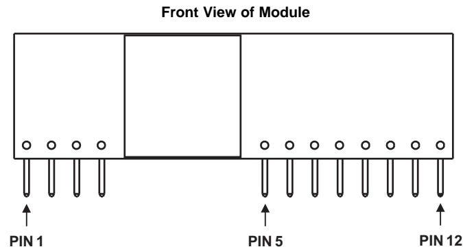
Figure 10. Pin/Terminal Locations
