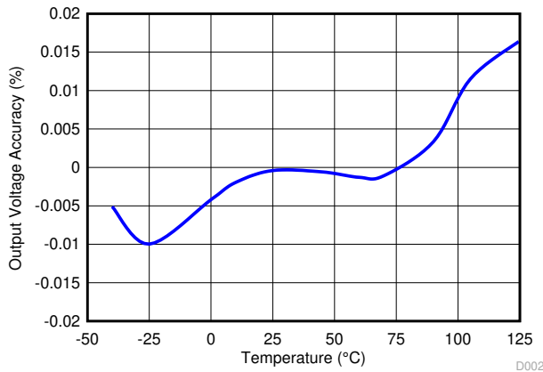
Figure 6-3. Output Voltage Accuracy vs Temperature
