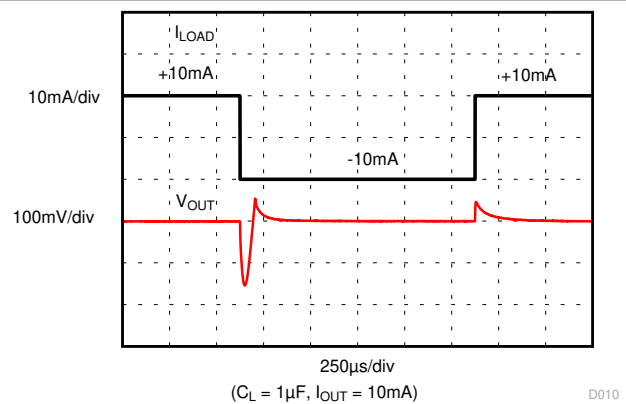
Figure 6-12. Load Transient
