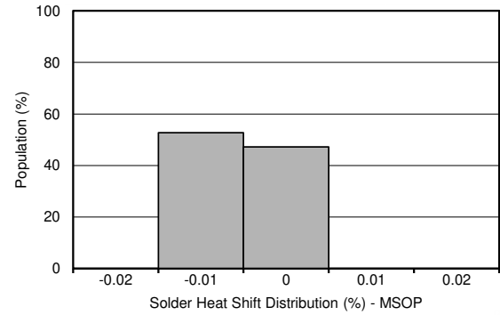
Figure 7-4. Solder Heat Shift Distribution (%), VSSOP Package
