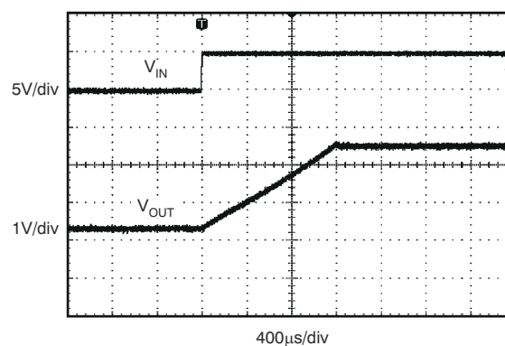
REF5025, C_L = 10\mu\text{F}
