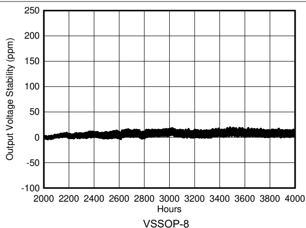
Figure 6-26. REF50xx Long-Term Stability (Second 2000 Hours)
