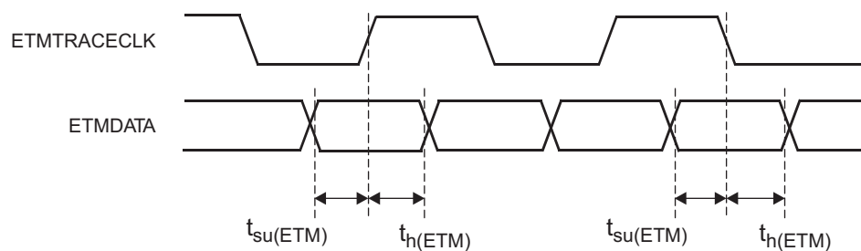
Figure 6-31. ETMDATA Timing
