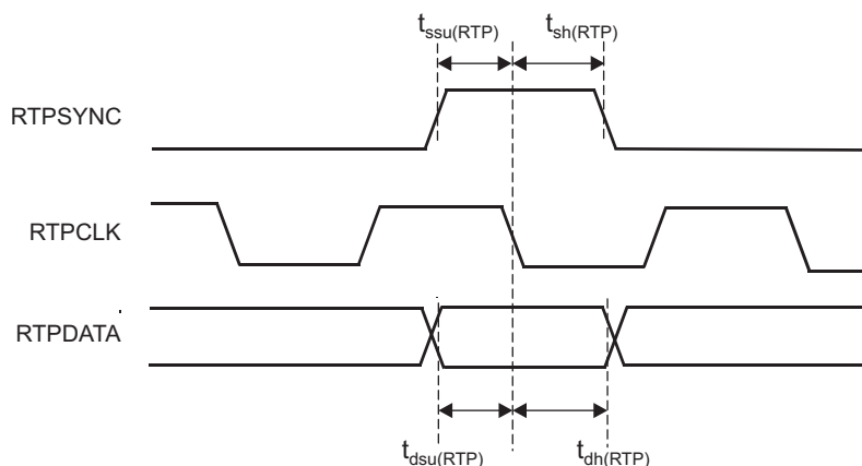
Figure 6-33. RTPDATA Timing
