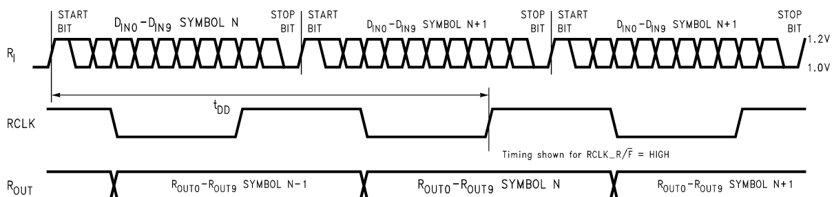
Figure 14. Deserializer Delay
