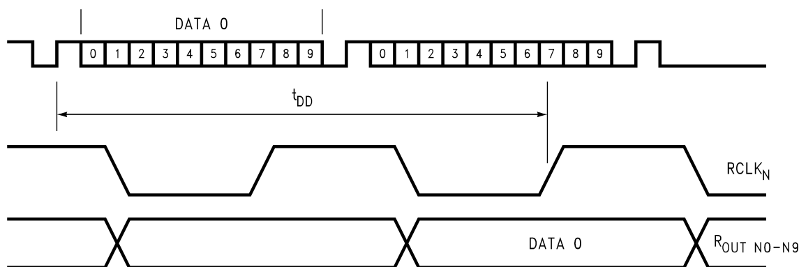
Figure 1. Deserializer Delay t DD
