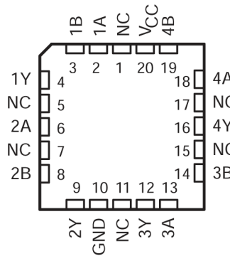
Figure 3-3. SN54AC08 FK Package (Top View)
