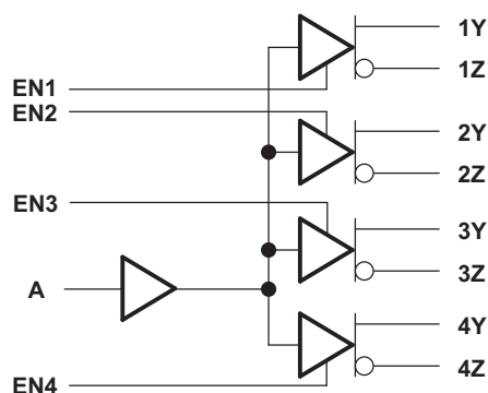
Figure 24. Example of Functional Block Diagram (SN65LVDS105)
