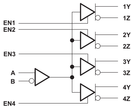
Figure 23. Example of Functional Block Diagram (SN65LVDS104)
