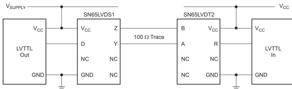
Simplified Schematic
