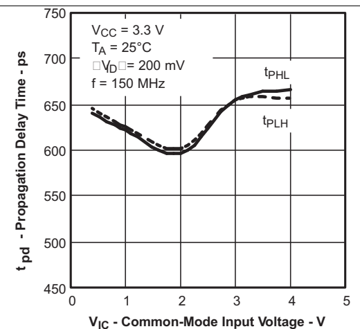
Figure 5. SN65LVDS101 Propagation Delay Time vs Common-Mode Input Voltage
